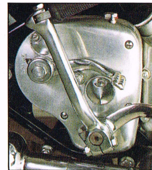
Foot-operated neutral lever. At whatever gear your Bullet is running, you can bring it back to neutral. All it takes is a gentle press of the lever.
