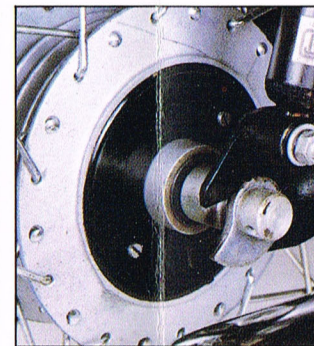
Changing tyres on the Bullet takes just minutes – the quickly detachable rear wheel assembly makes sure!
